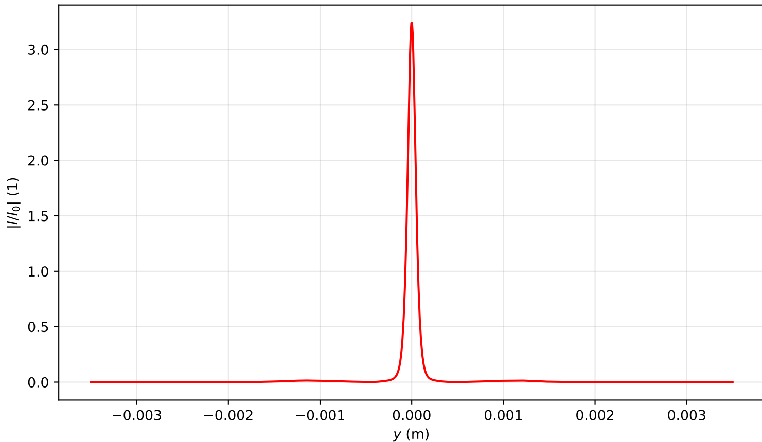
Intensity profile I(x=0, y, z=3.344)/I_0 , P_{in}=14.0P_{cr} , artificial time
