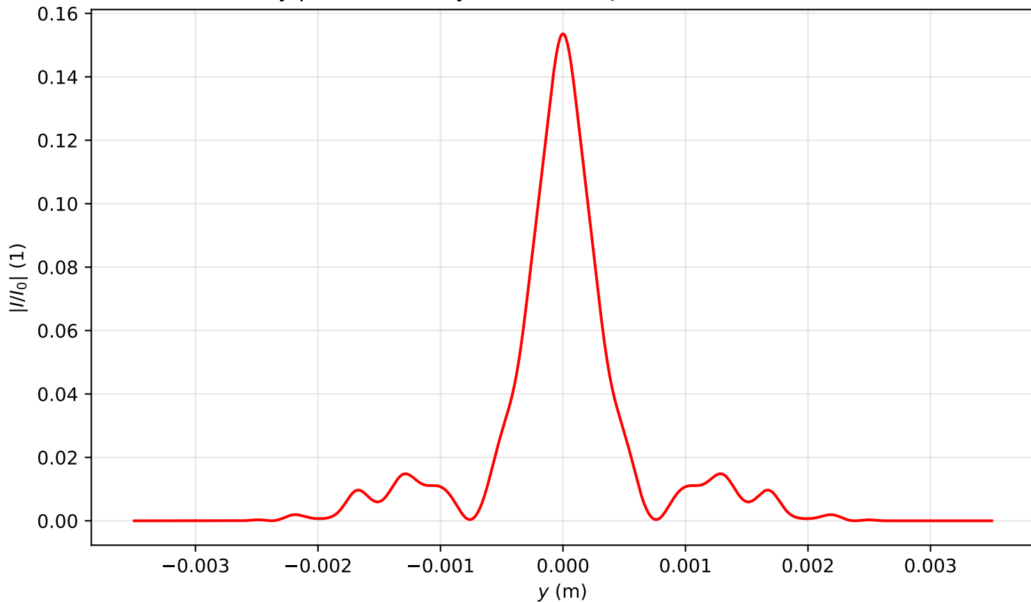
Intensity profile I(x = 0, y, z = 3.821)/I_0 , P_{in}=14.0P_{cr} , artificial time
