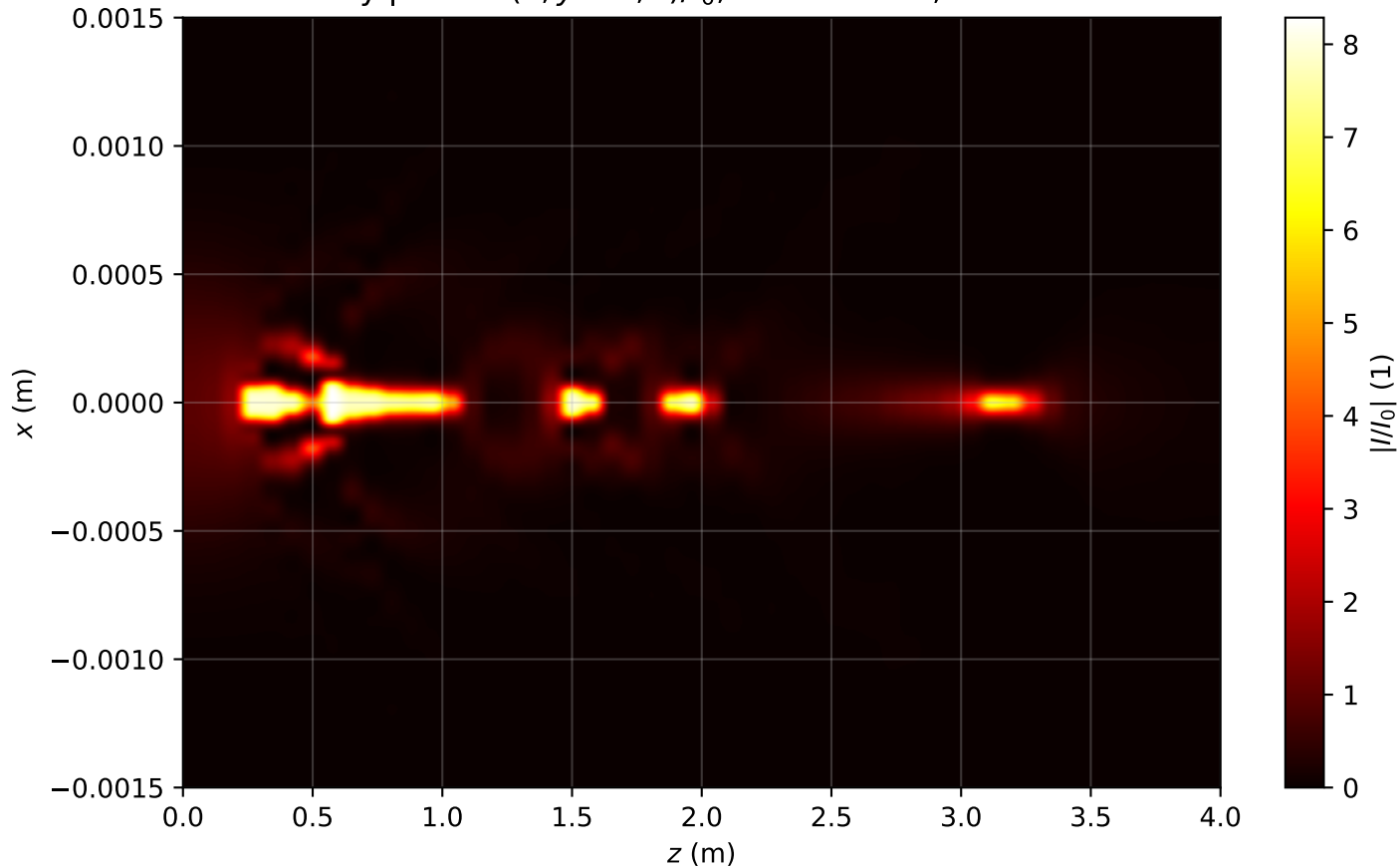
Intensity profile I(x, y = 0, z)/I_0 , P_{in}=14.0P_{cr} , artificial time
