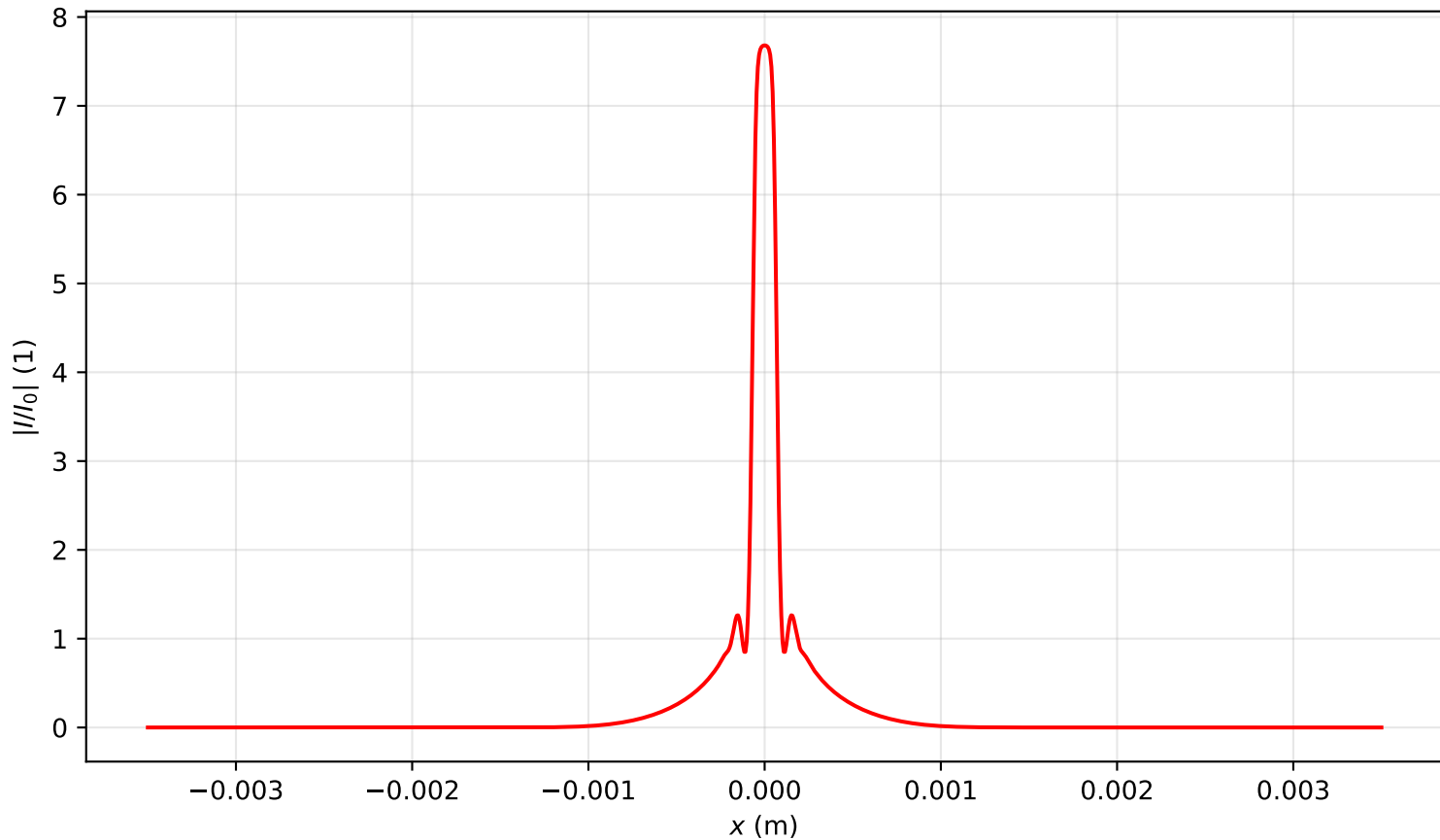
Intensity profile I(x, y = 0, z = 0.239)/I_0 , P_{in}=14.5P_{cr} , artificial time
