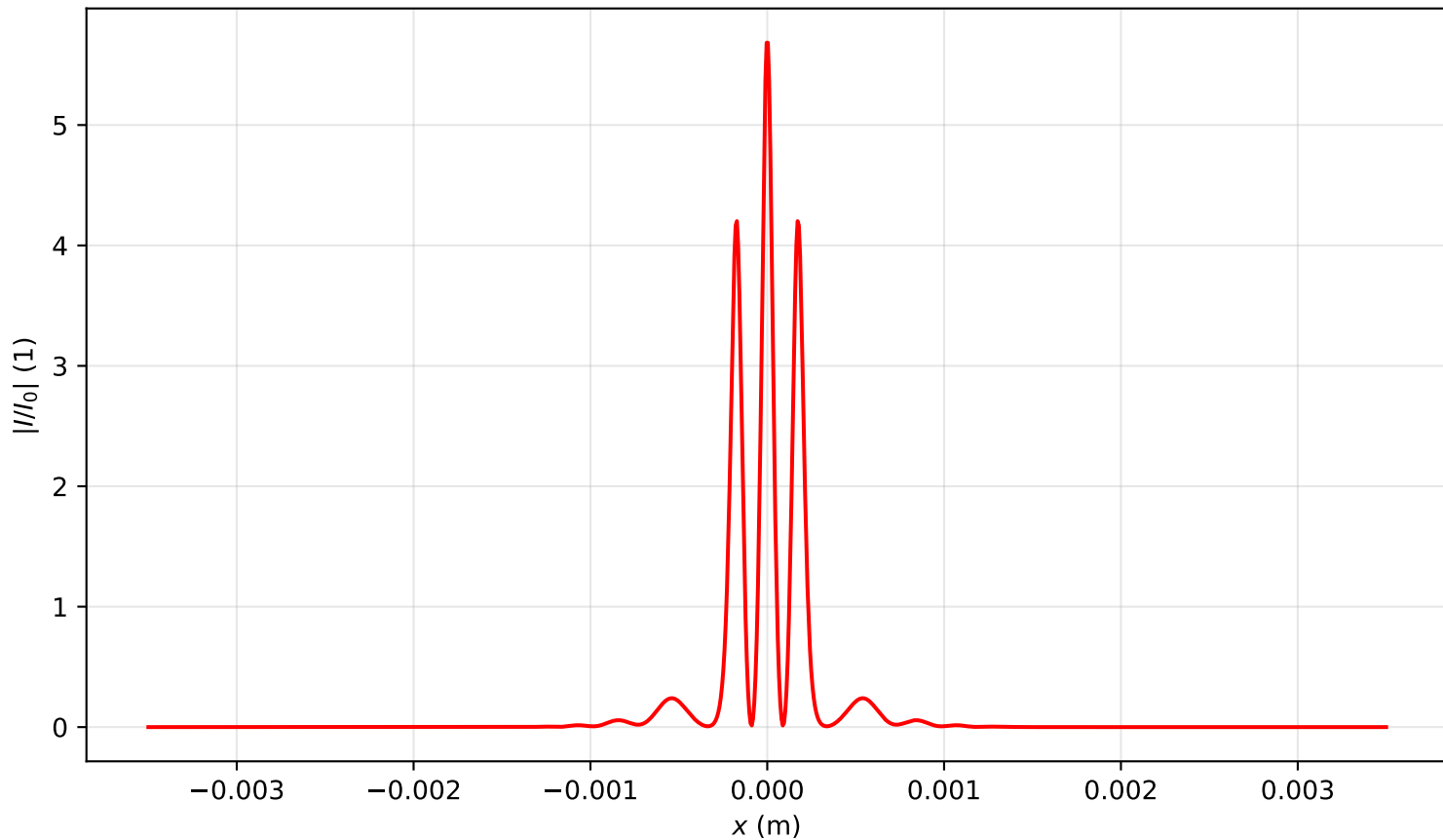
Intensity profile I(x, y = 0, z = 0.478)/I_0 , P_{in}=14.5P_{cr} , artificial time
