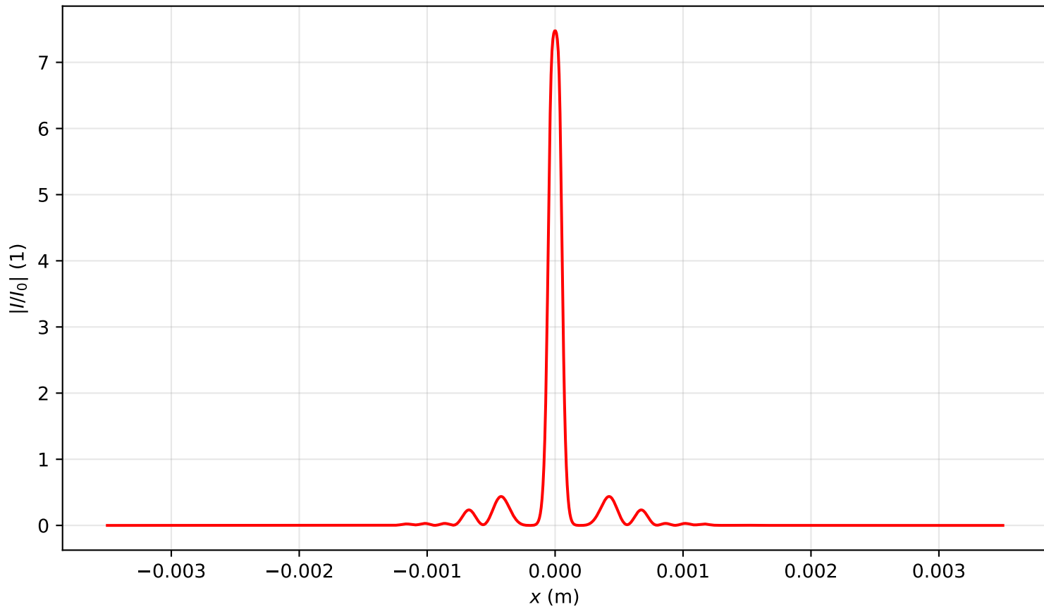
Intensity profile I(x, y = 0, z = 0.716)/I_0 , P_{in}=14.5P_{cr} , artificial time
