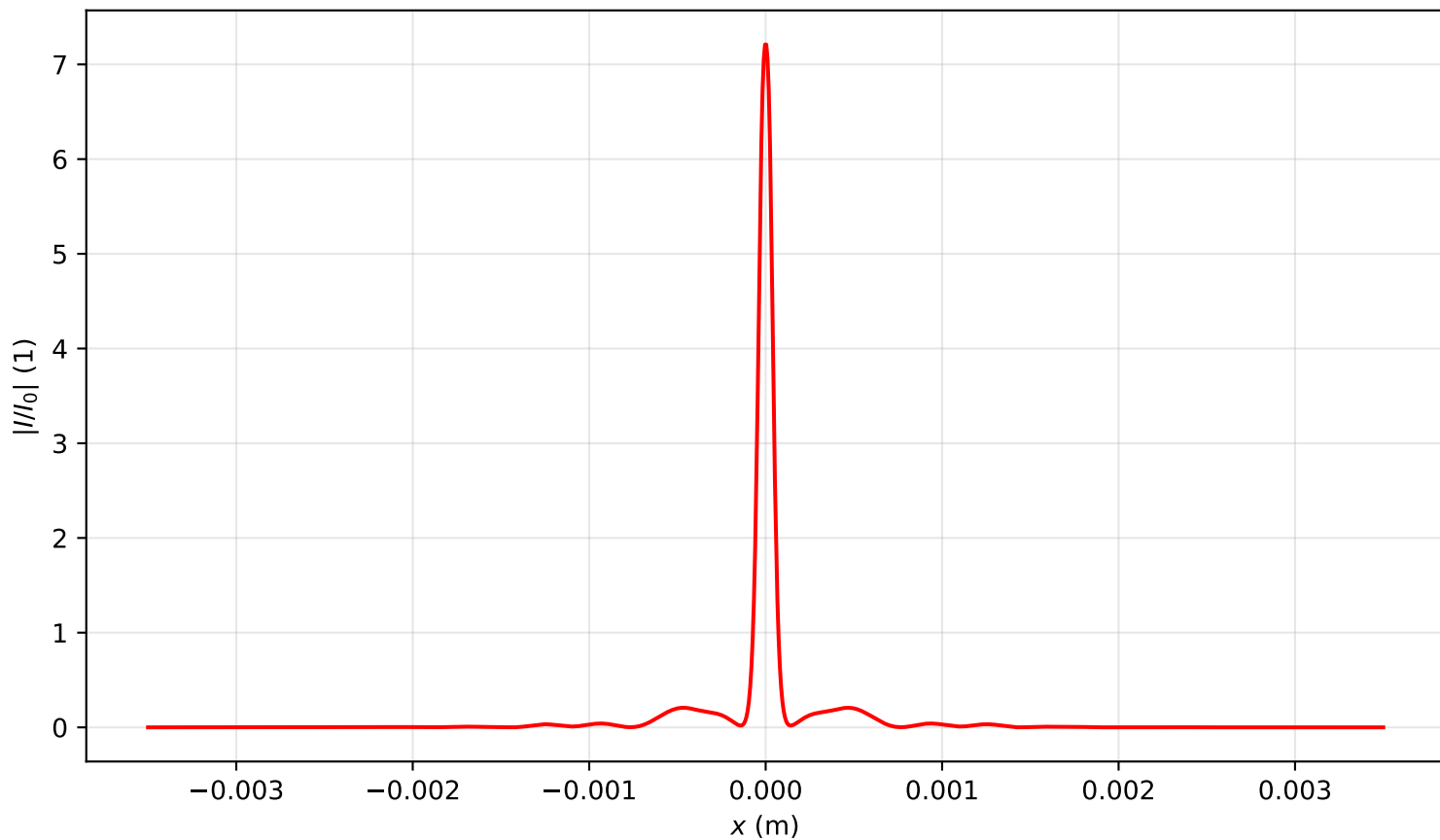
Intensity profile I(x, y = 0, z = 0.955)/I_0 , P_{in}=14.5P_{cr} , artificial time
