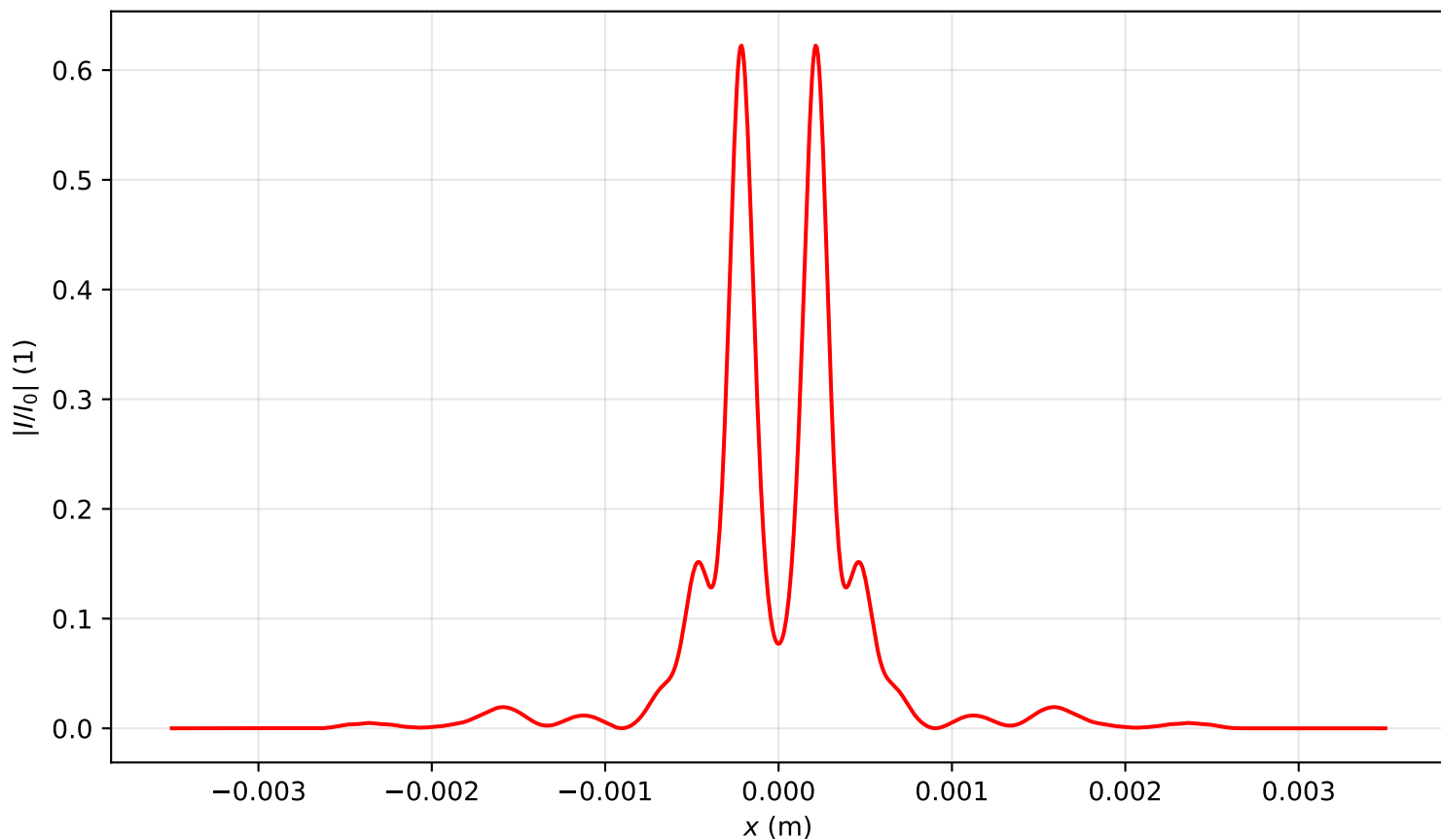
Intensity profile I(x, y = 0, z = 1.194)/I_0 , P_{in}=14.5P_{cr} , artificial time
