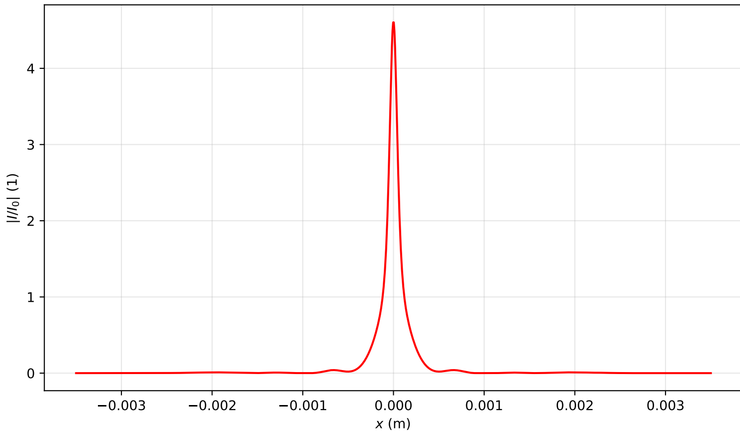
Intensity profile I(x, y = 0, z = 1.433)/I_0 , P_{in}=14.5P_{cr} , artificial time
