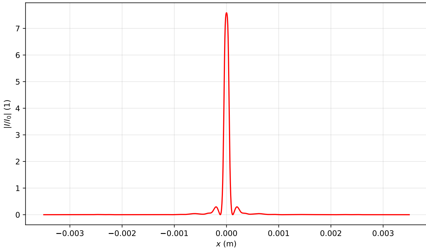
Intensity profile I(x, y = 0, z = 1.911)/I_0 , P_{in}=14.5P_{cr} , artificial time
