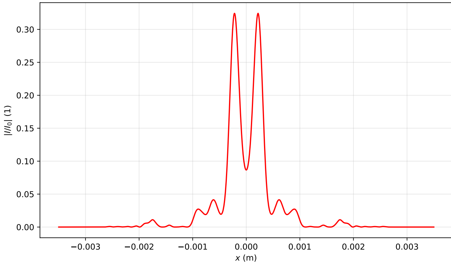
Intensity profile I(x, y = 0, z = 2.149)/I_0 , P_{in}=14.5P_{cr} , artificial time
