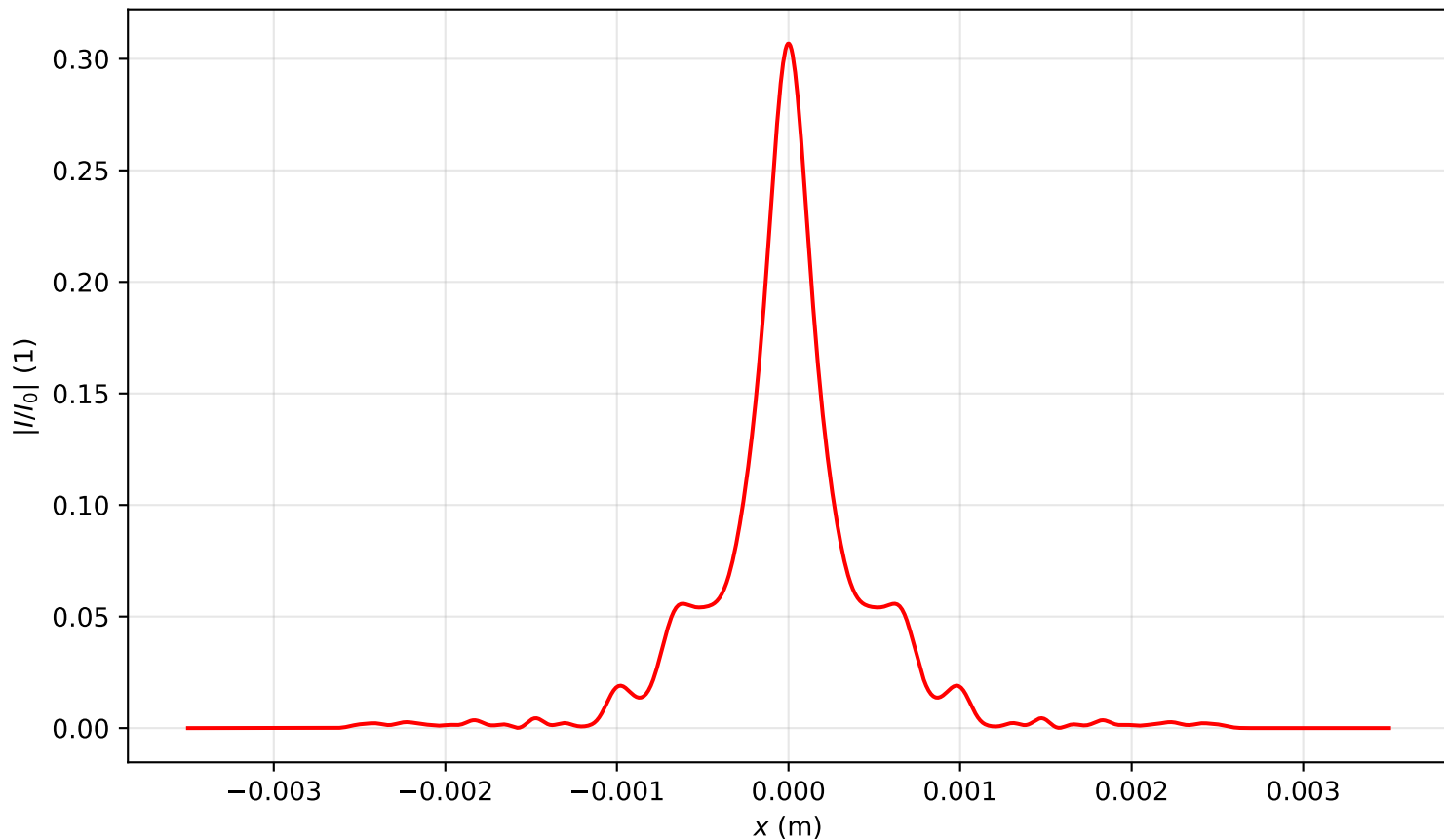
Intensity profile I(x, y = 0, z = 2.388)/I_0 , P_{in}=14.5P_{cr} , artificial time
