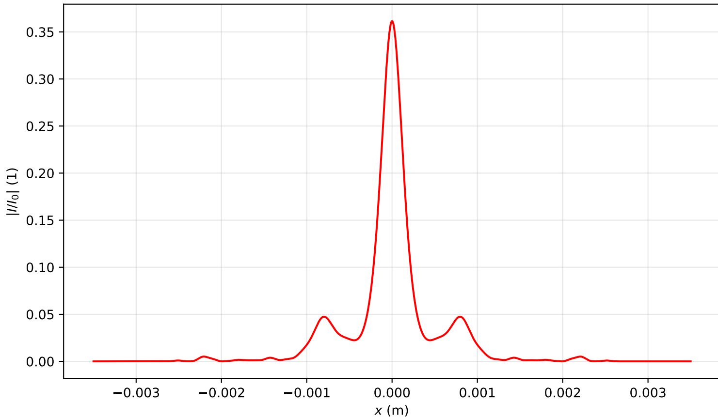
Intensity profile I(x, y = 0, z = 2.627)/I_0 , P_{in}=14.5P_{cr} , artificial time
