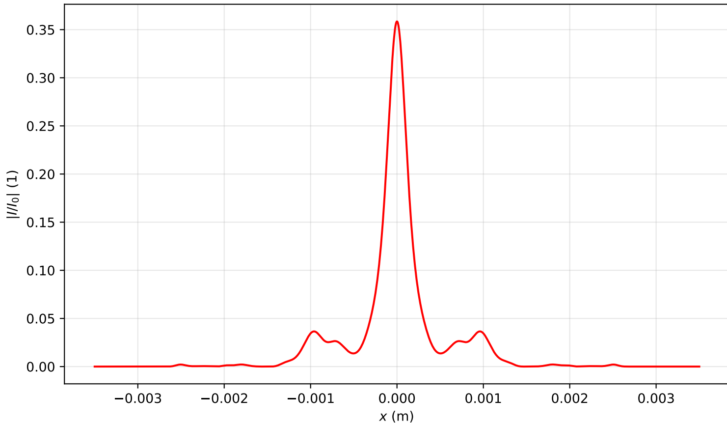
Intensity profile I(x, y = 0, z = 2.866)/I_0 , P_{in}=14.5P_{cr} , artificial time
