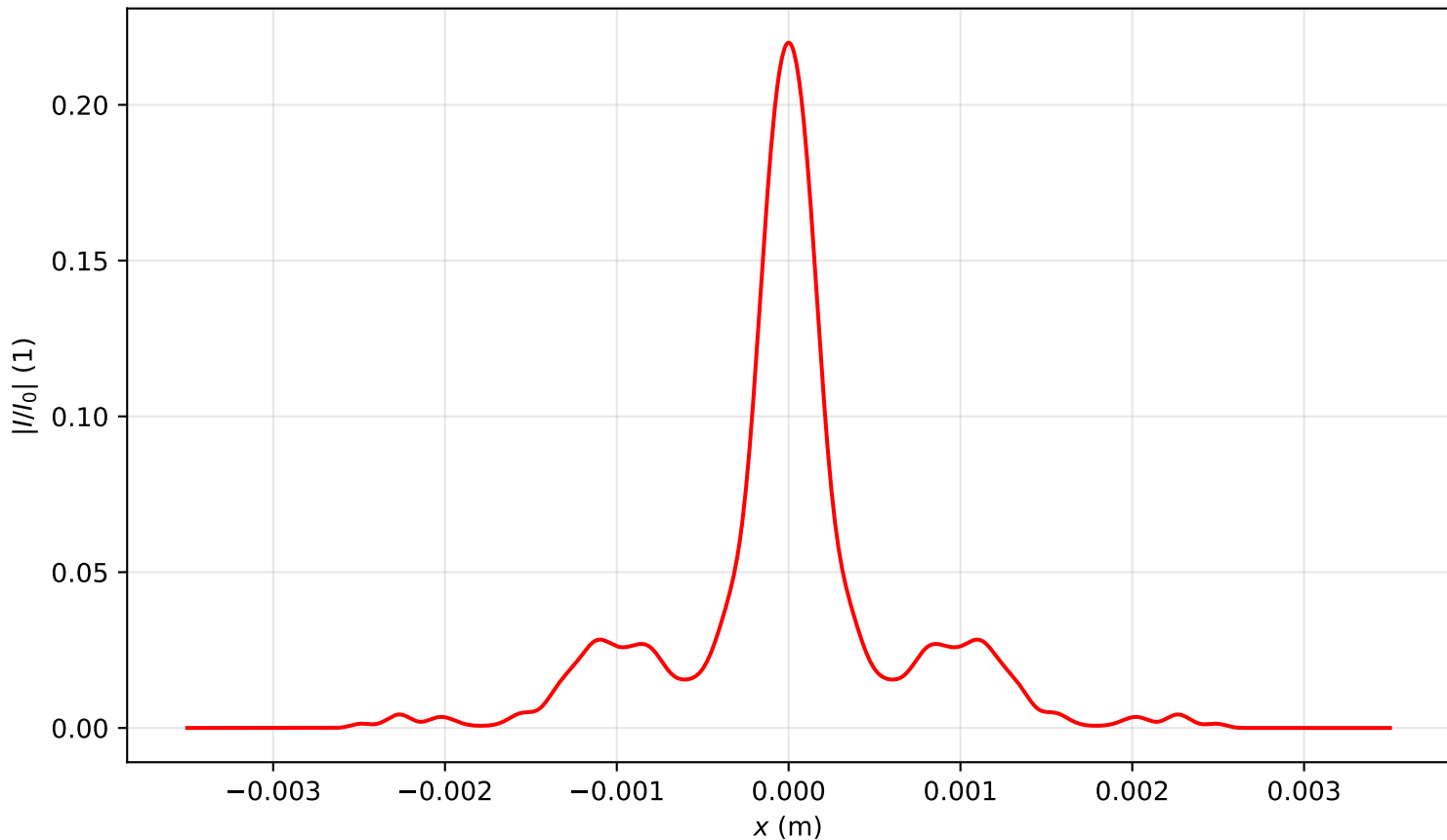
Intensity profile I(x, y = 0, z = 3.105)/I_0 , P_{in}=14.5P_{cr} , artificial time
