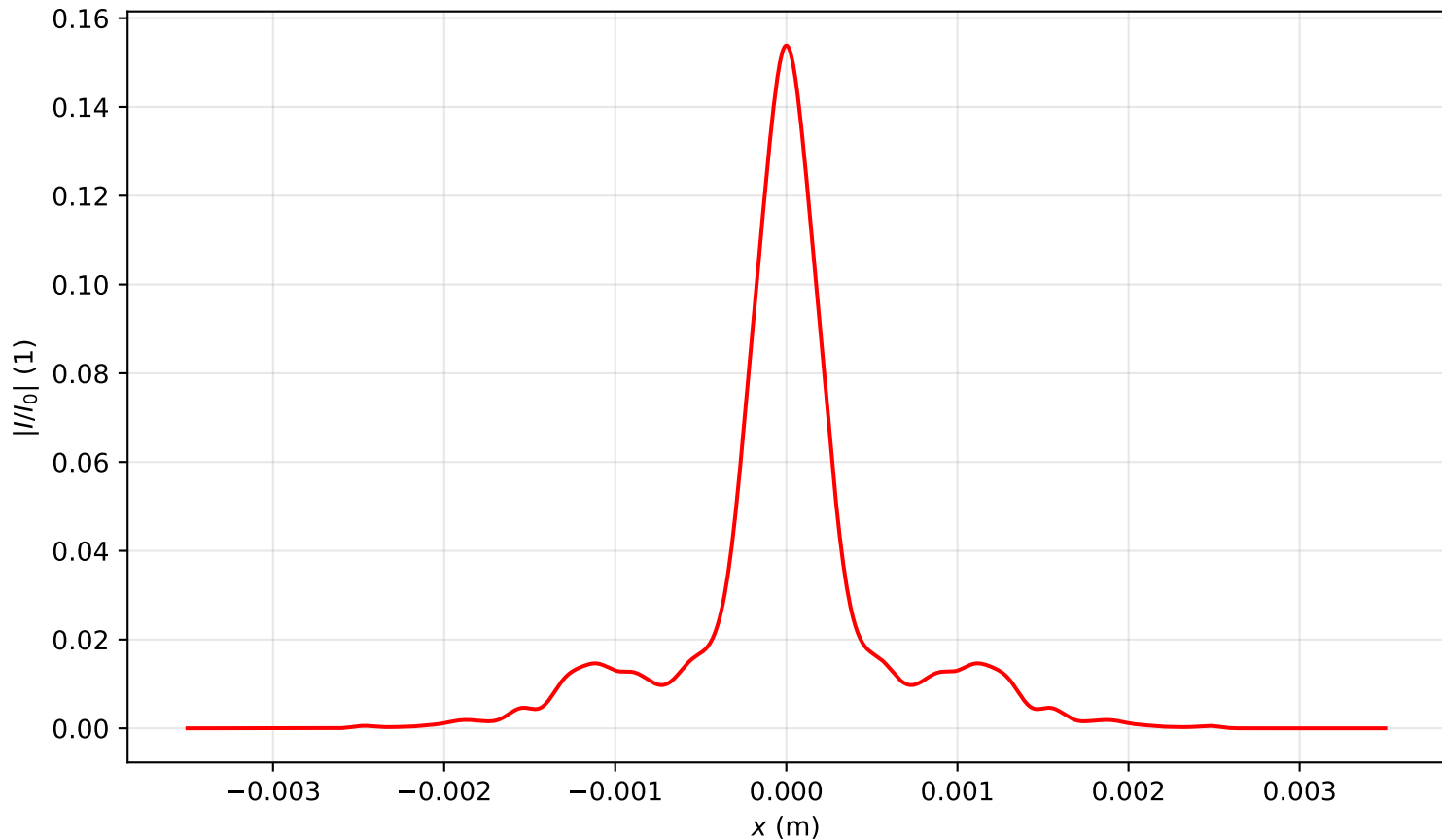
Intensity profile I(x, y = 0, z = 3.344)/I_0 , P_{in}=14.5P_{cr} , artificial time
