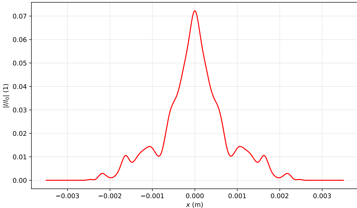
Intensity profile I(x, y = 0, z = 3.821)/I_0 , P_{in}=14.5P_{cr} , artificial time
