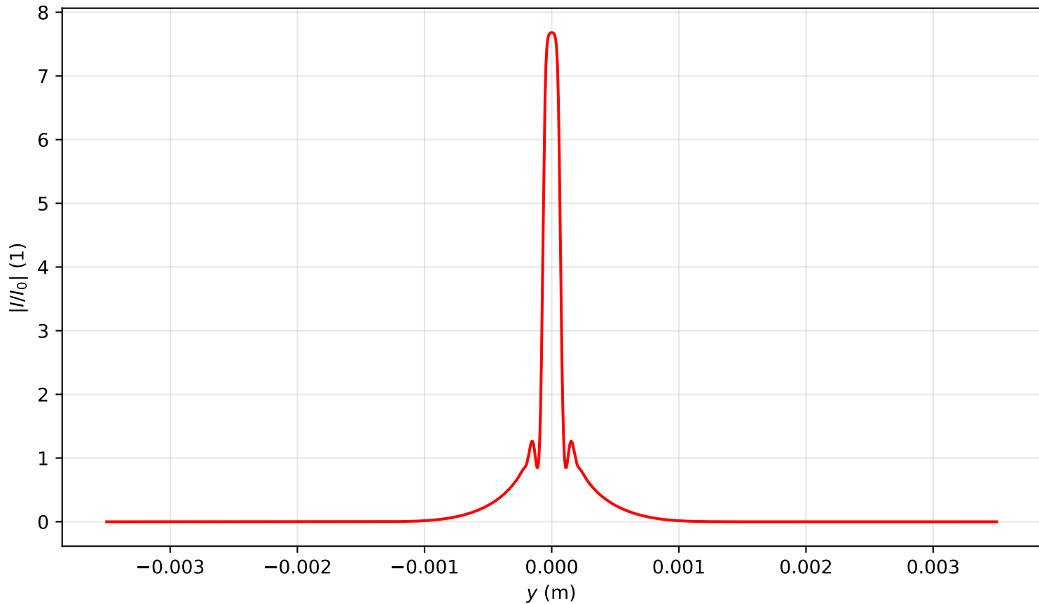
Intensity profile I(x=0, y, z=0.239)/I_0 , P_{in}=14.5P_{cr} , artificial time
