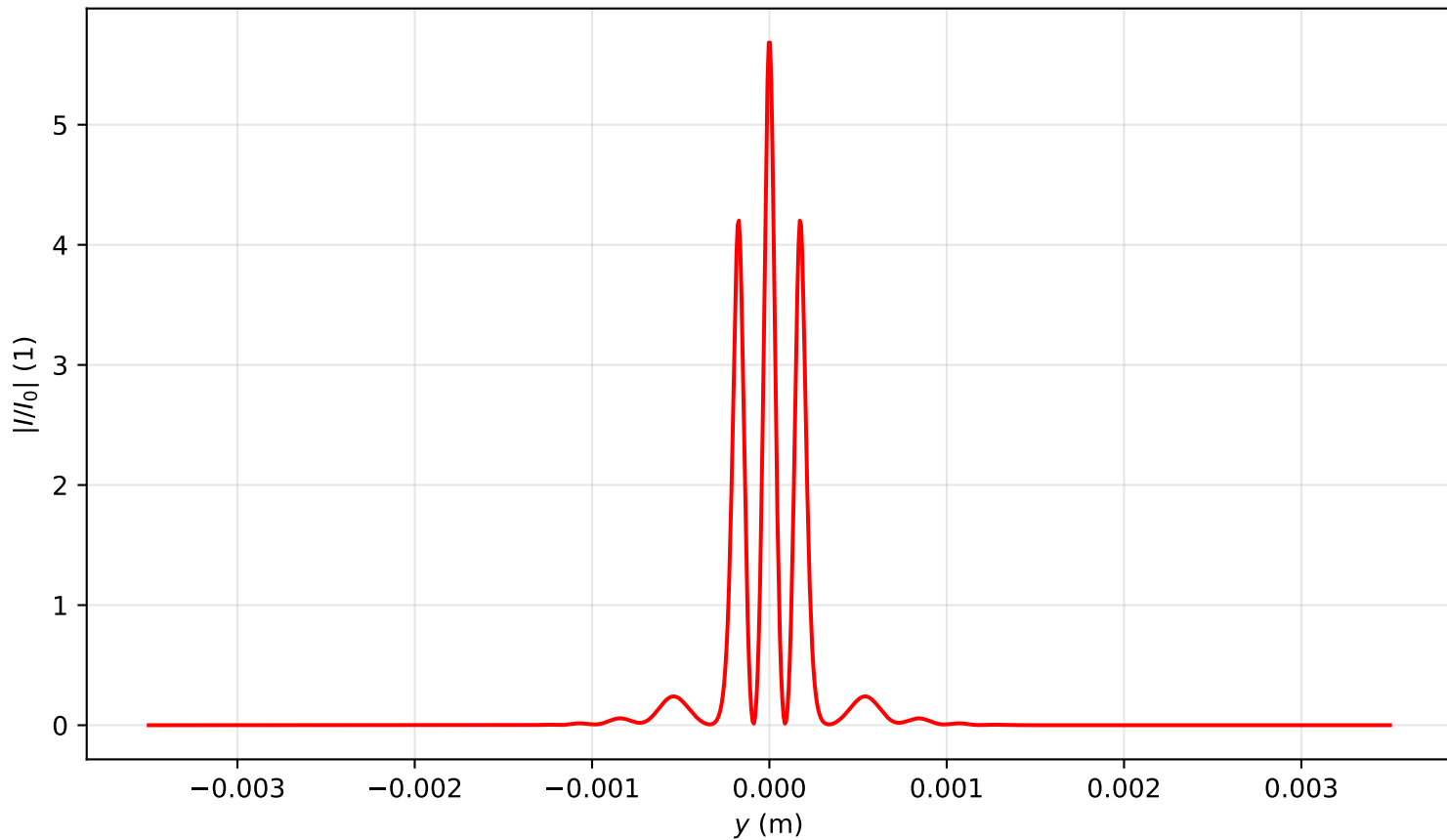
Intensity profile I(x=0, y, z=0.478)/I_0 , P_{in}=14.5P_{cr} , artificial time
