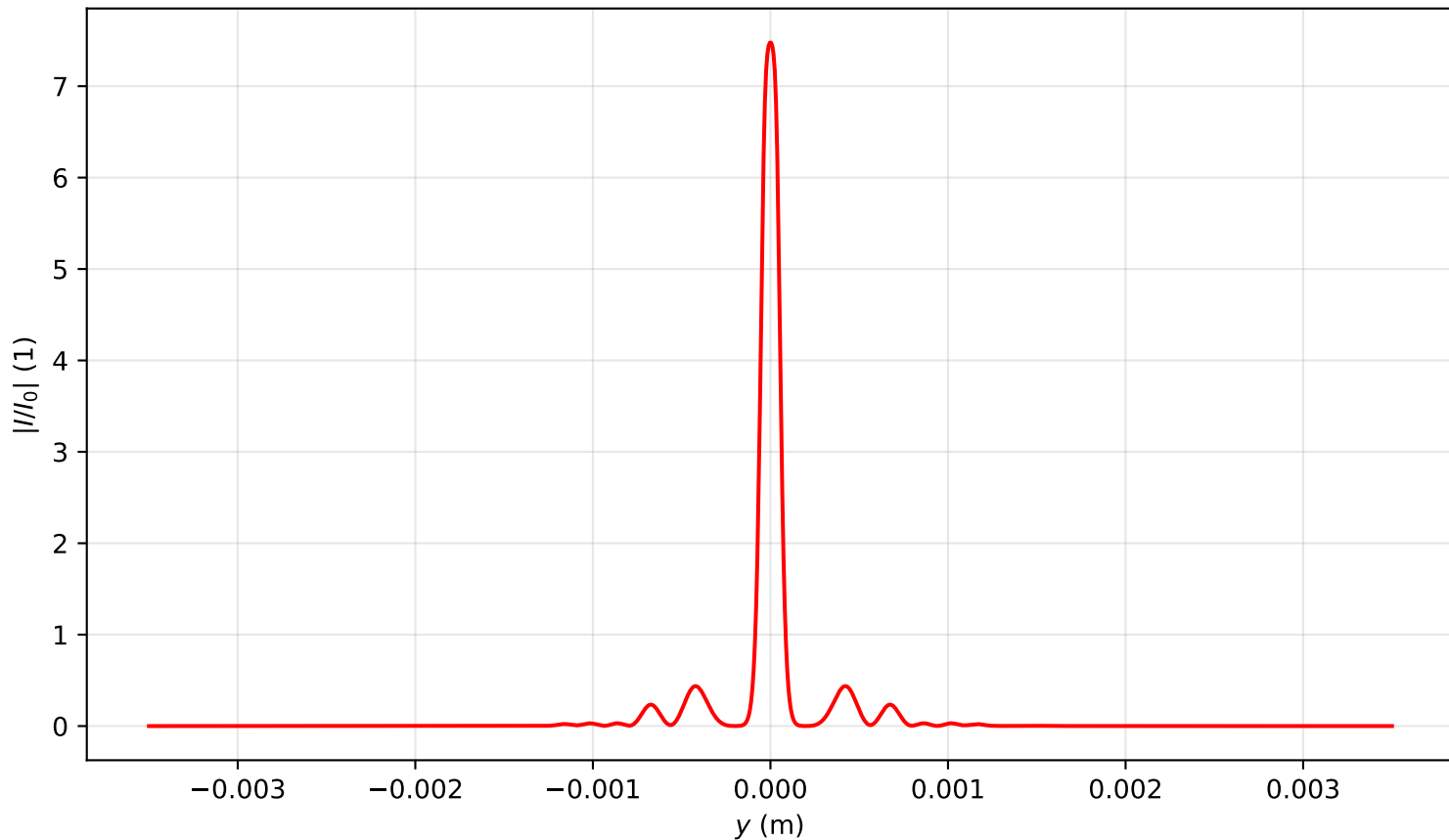
Intensity profile I(x=0, y, z=0.716)/I_0 , P_{in}=14.5P_{cr} , artificial time
