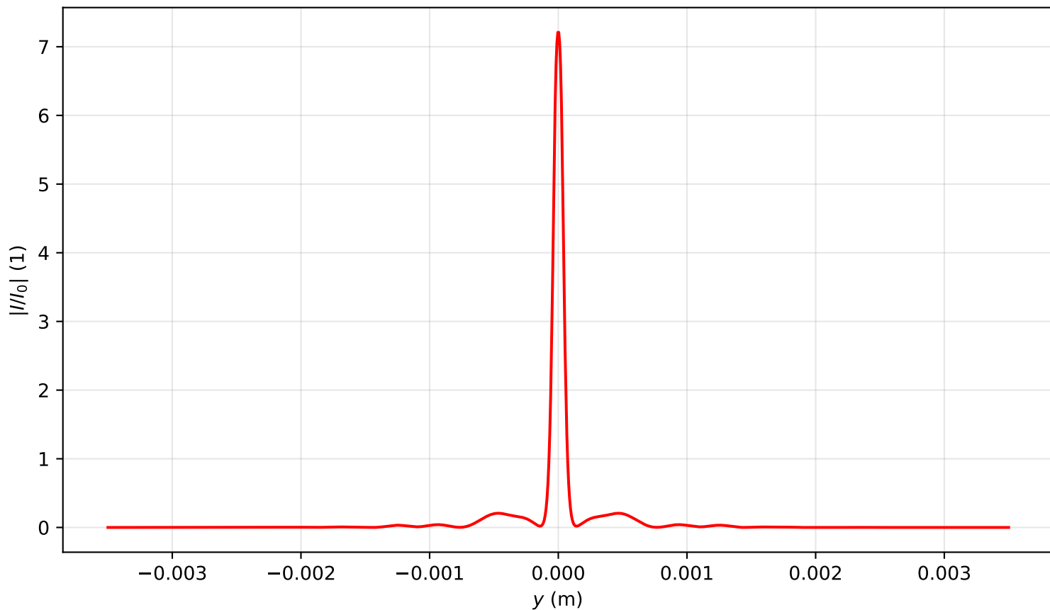
Intensity profile I(x=0, y, z=0.955)/I_0 , P_{in}=14.5P_{cr} , artificial time
