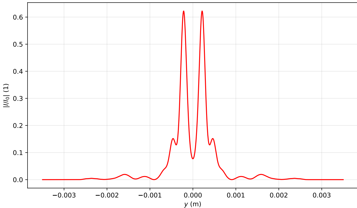
Intensity profile I(x=0, y, z=1.194)/I_0 , P_{in}=14.5P_{cr} , artificial time
