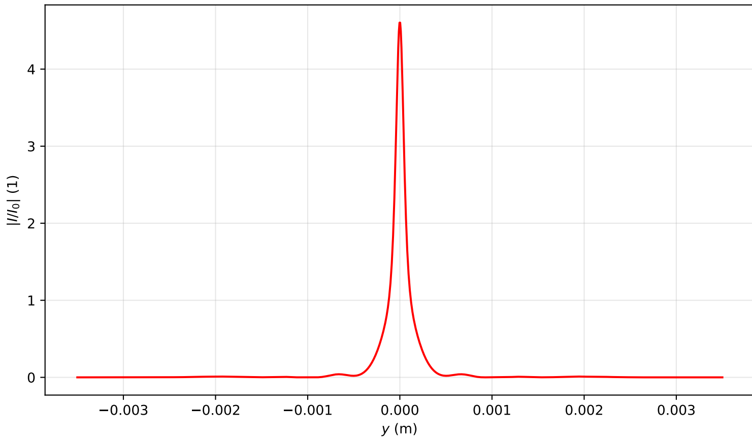
Intensity profile I(x=0, y, z=1.433)/I_0 , P_{in}=14.5P_{cr} , artificial time
