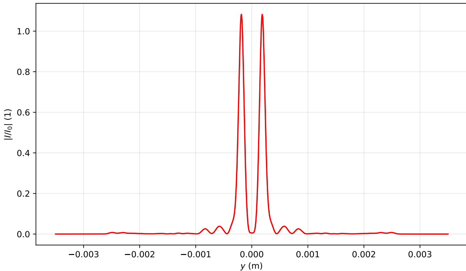
Intensity profile I(x=0, y, z=1.672)/I_0 , P_{in}=14.5P_{cr} , artificial time
