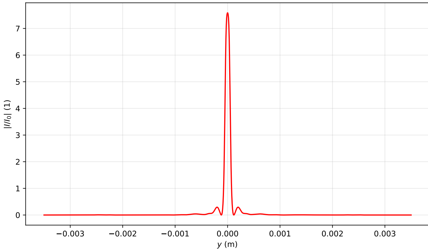
Intensity profile I(x=0, y, z=1.911)/I_0 , P_{in}=14.5P_{cr} , artificial time
