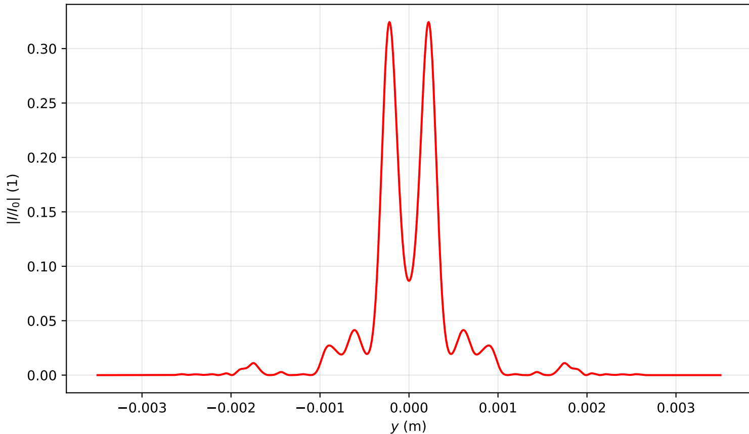
Intensity profile I(x = 0, y, z = 2.149)/I_0 , P_{in}=14.5P_{cr} , artificial time
