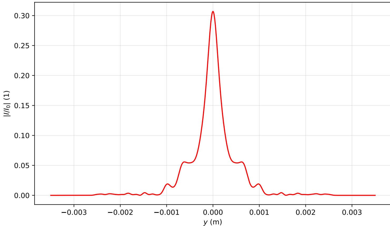
Intensity profile I(x = 0, y, z = 2.388)/I_0 , P_{in}=14.5P_{cr} , artificial time
