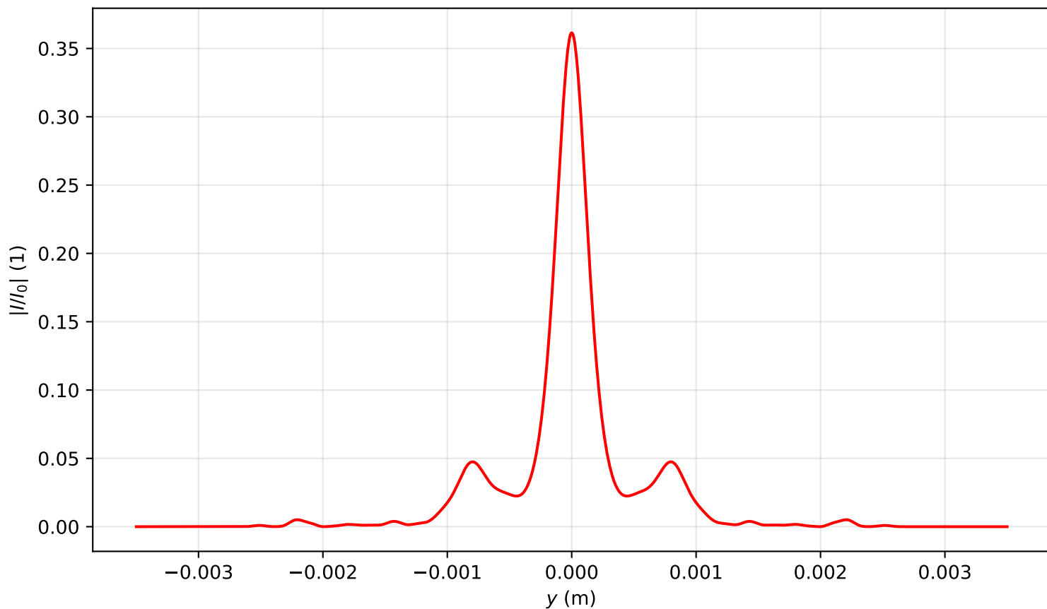
Intensity profile I(x=0, y, z=2.627)/I_0 , P_{in}=14.5P_{cr} , artificial time
