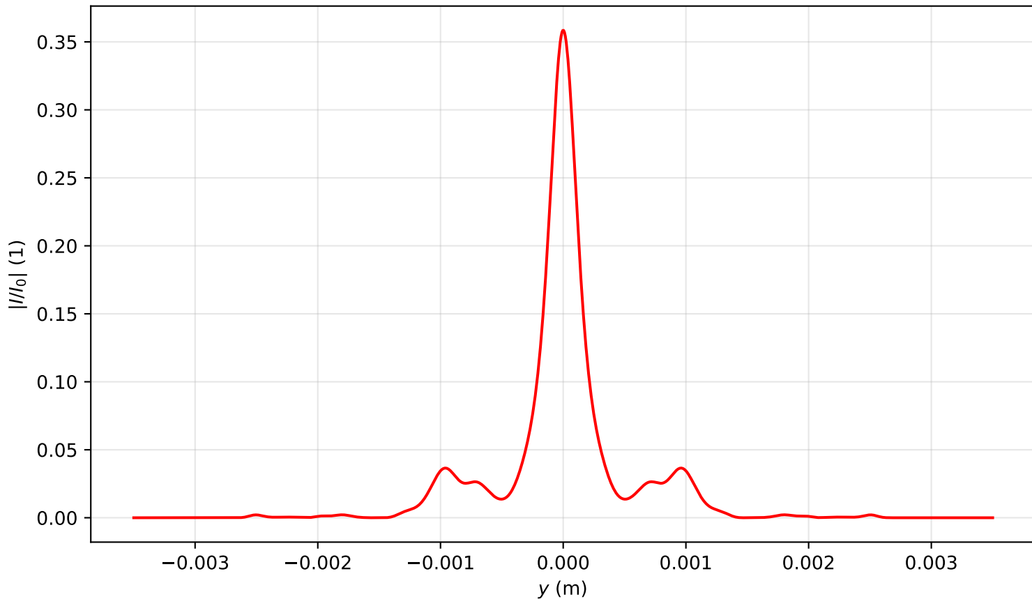
Intensity profile I(x=0, y, z=2.866)/I_0 , P_{in}=14.5P_{cr} , artificial time
