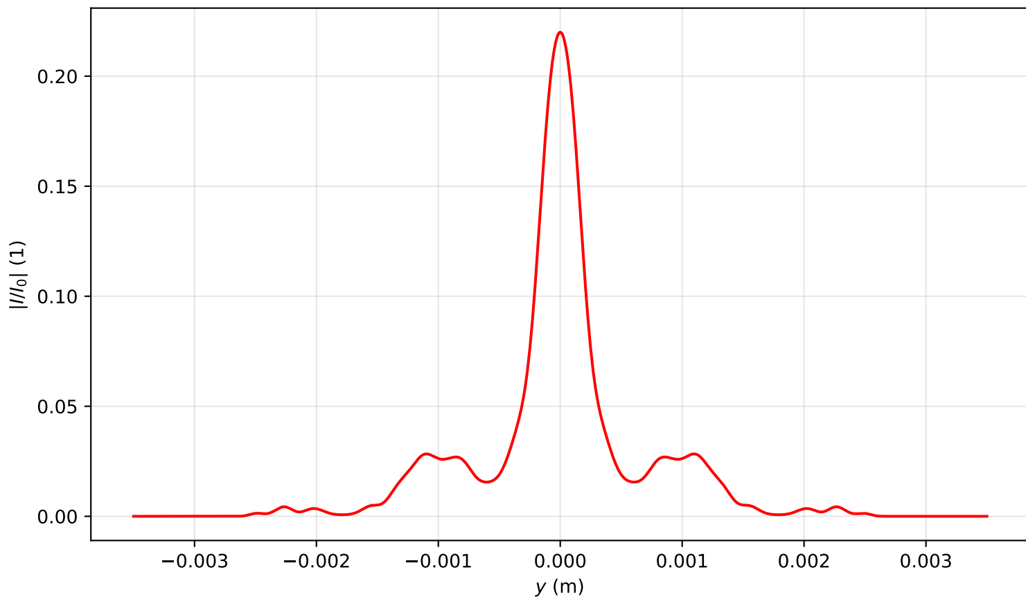
Intensity profile I(x = 0, y, z = 3.105)/I_0 , P_{in}=14.5P_{cr} , artificial time
