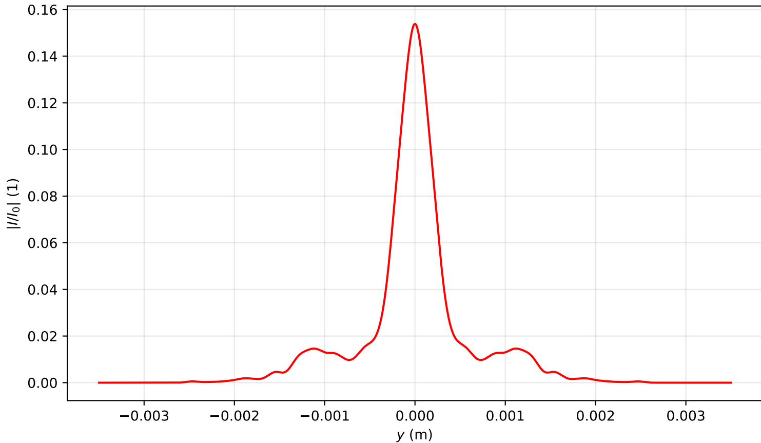
Intensity profile I(x=0, y, z=3.344)/I_0 , P_{in}=14.5P_{cr} , artificial time
