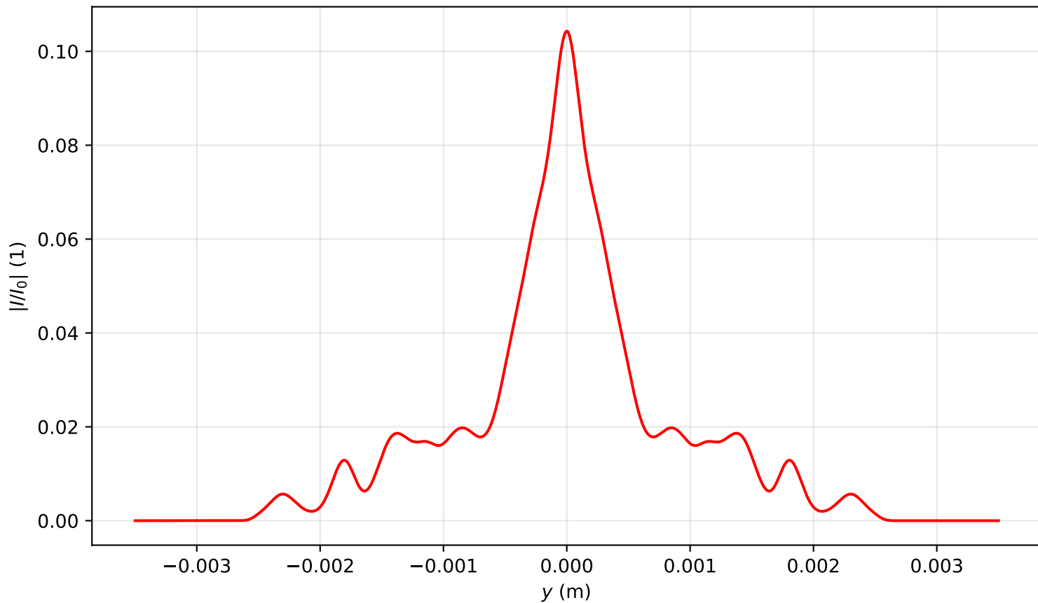
Intensity profile I(x = 0, y, z = 3.582)/I_0 , P_{in}=14.5P_{cr} , artificial time
