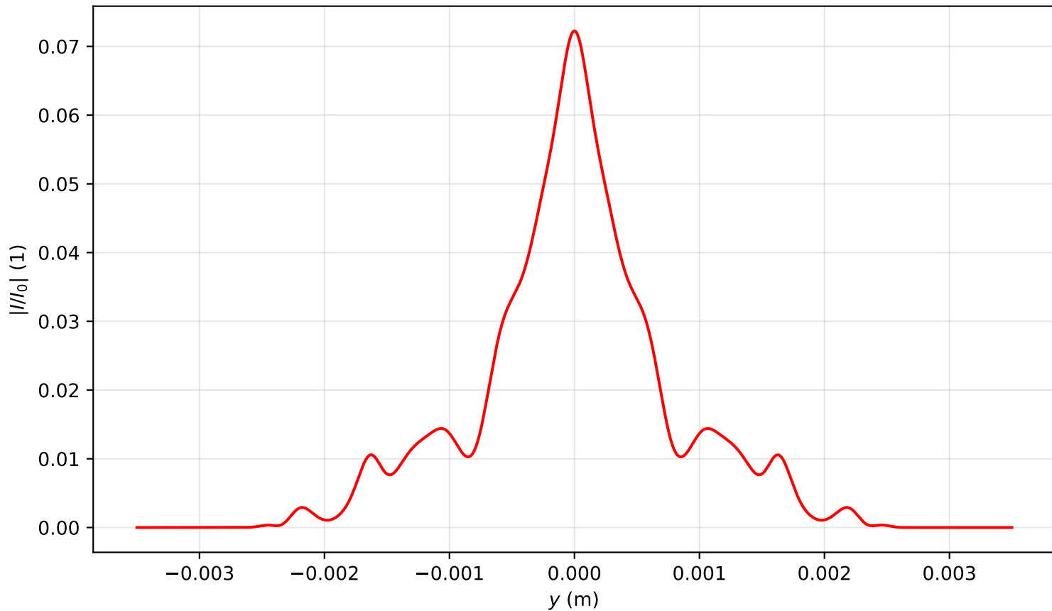
Intensity profile I(x=0, y, z=3.821)/I_0 , P_{in}=14.5P_{cr} , artificial time
