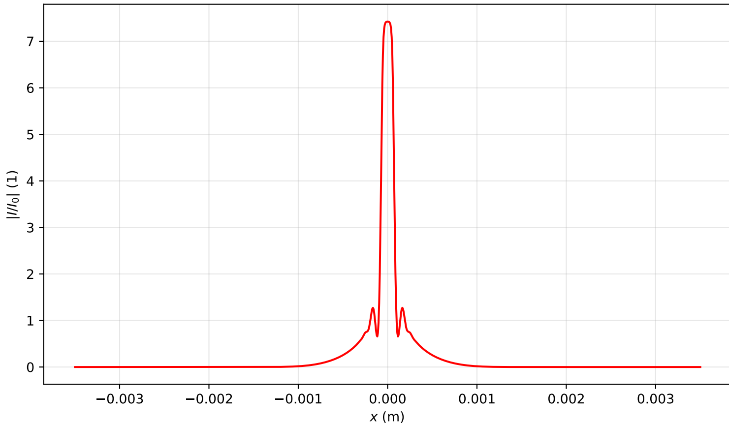
Intensity profile I(x, y = 0, z = 0.239)/I_0 , P_{in}=15.0P_{cr} , artificial time
