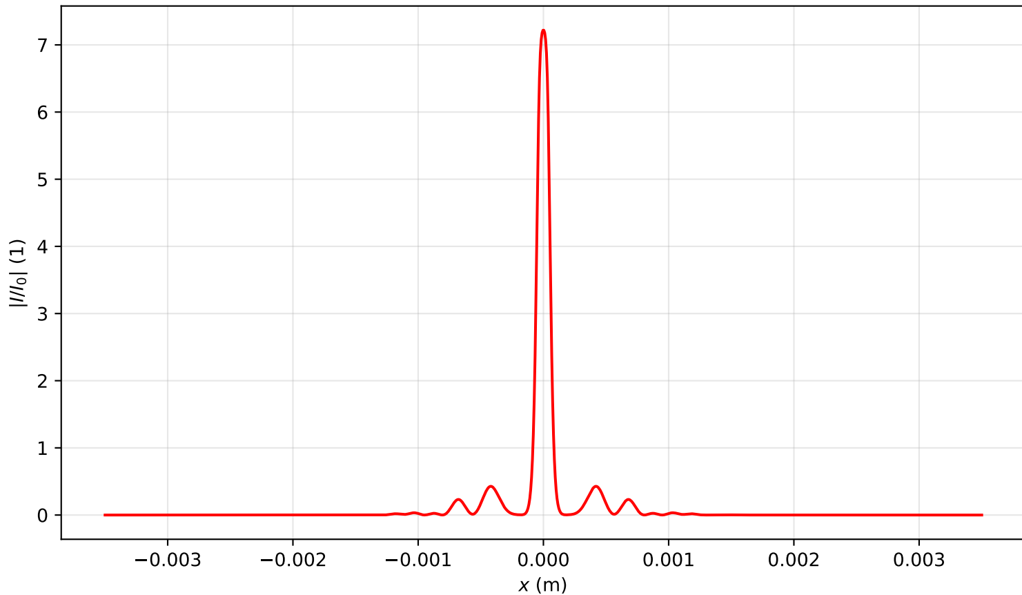
Intensity profile I(x, y = 0, z = 0.716)/I_0 , P_{in}=15.0P_{cr} , artificial time
