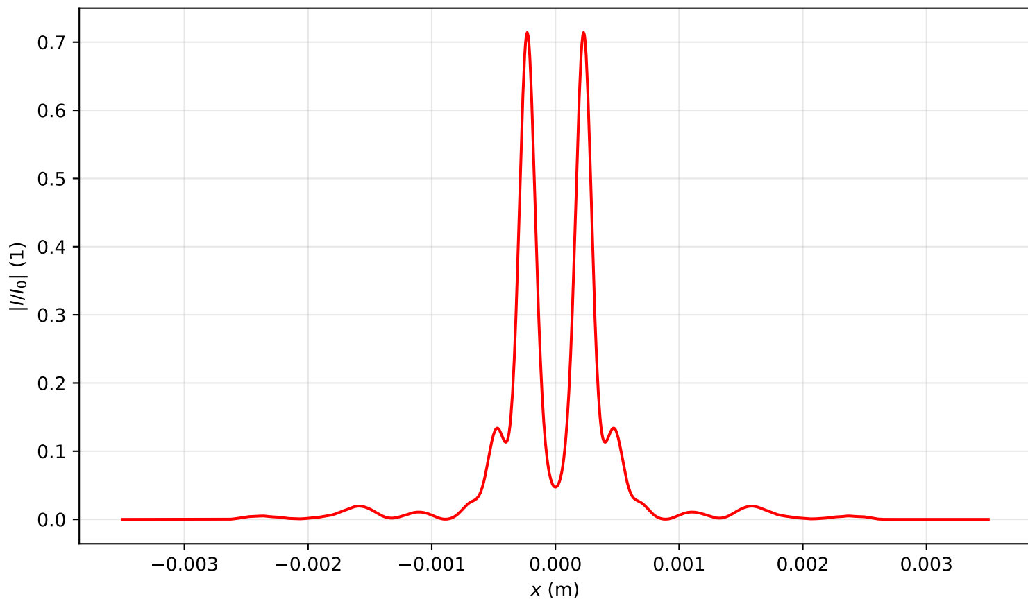
Intensity profile I(x, y = 0, z = 1.194)/I_0 , P_{in}=15.0P_{cr} , artificial time
