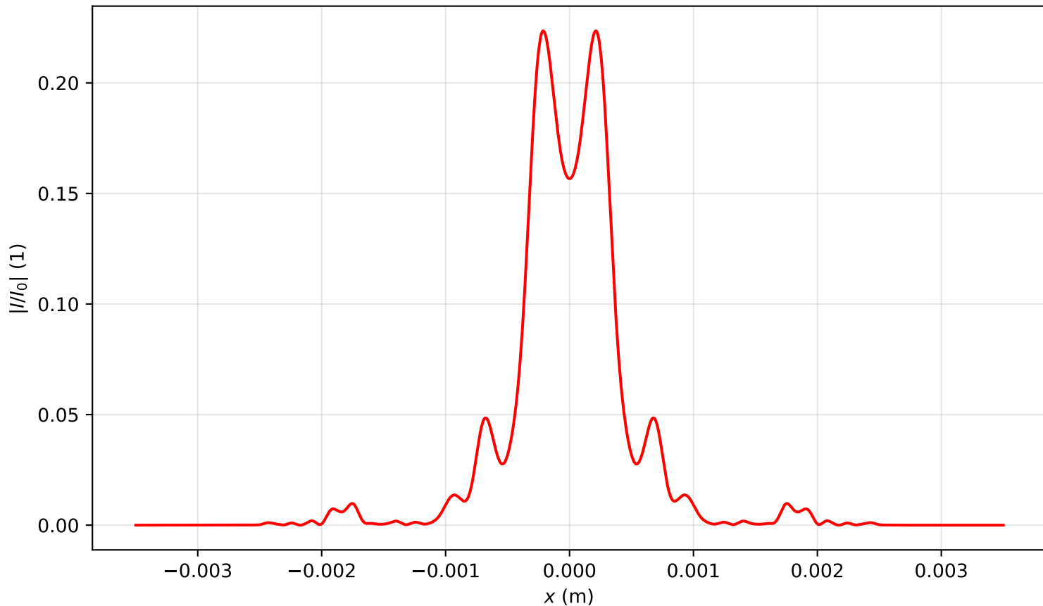
Intensity profile I(x, y = 0, z = 2.149)/I_0 , P_{in}=15.0P_{cr} , artificial time
