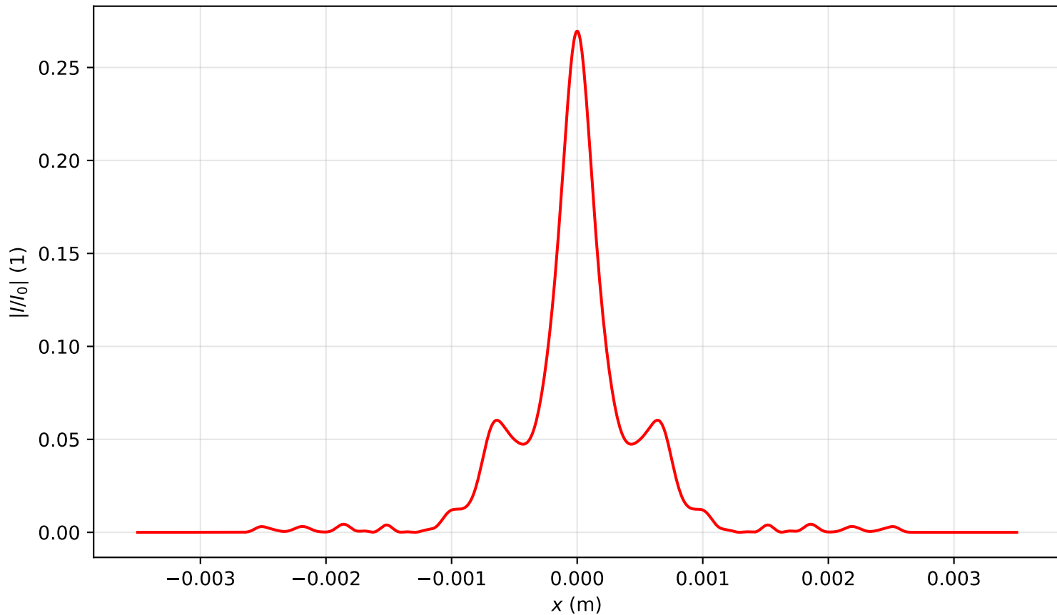
Intensity profile I(x, y = 0, z = 2.388)/I_0 , P_{in}=15.0P_{cr} , artificial time
