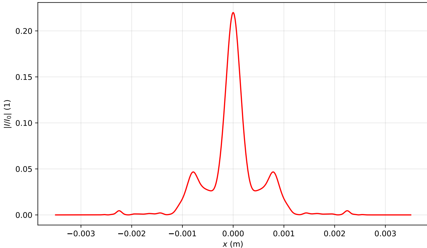
Intensity profile I(x, y = 0, z = 2.627)/I_0 , P_{in}=15.0P_{cr} , artificial time
