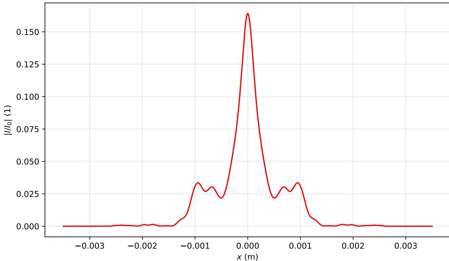
Intensity profile I(x, y = 0, z = 2.866)/I_0 , P_{in}=15.0P_{cr} , artificial time
