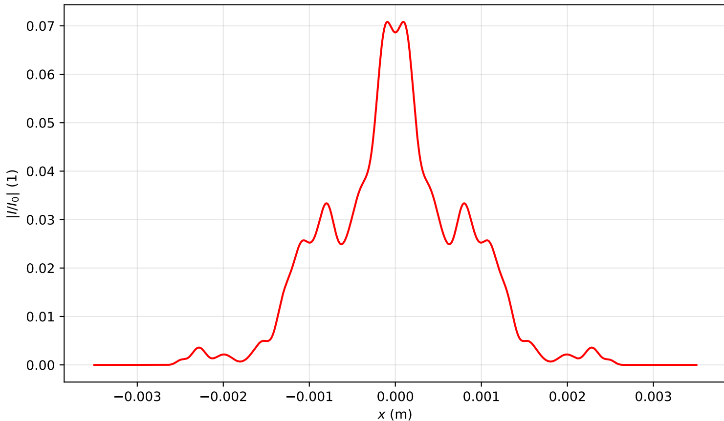
Intensity profile I(x, y = 0, z = 3.105)/I_0 , P_{in}=15.0P_{cr} , artificial time
