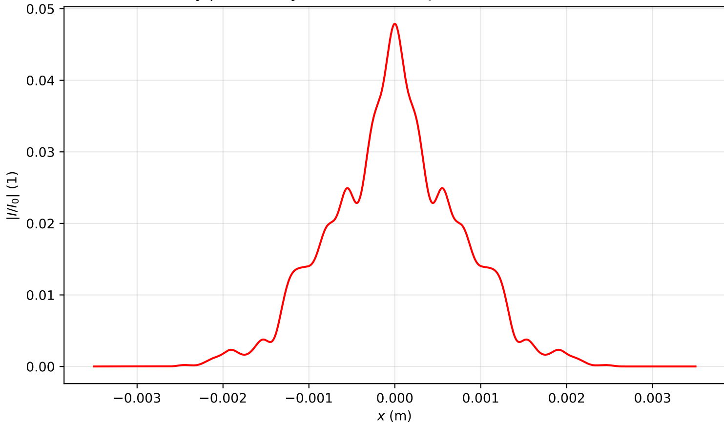
Intensity profile I(x, y = 0, z = 3.344)/I_0 , P_{in}=15.0\text{Pcr} , artificial time
