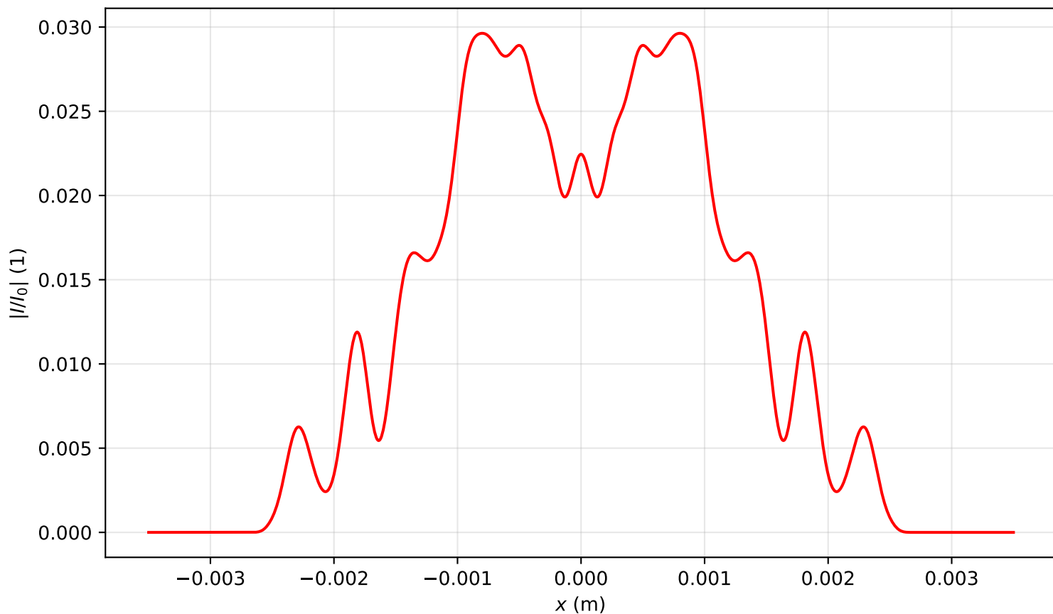
Intensity profile I(x, y = 0, z = 3.582)/I_0 , P_{in}=15.0\text{Pcr} , artificial time
