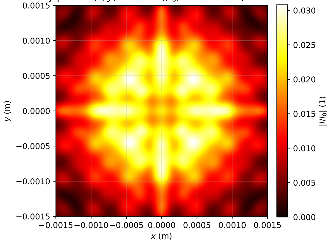
Intensity profile I(x, y, z = 3.582)/I_0 , P_{in}=15.0P_{cr} , artificial time
