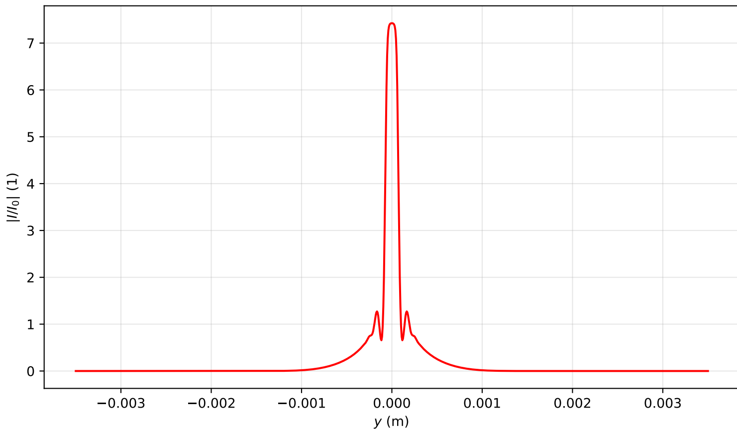
Intensity profile I(x=0, y, z=0.239)/I_0 , P_{in}=15.0P_{cr} , artificial time
