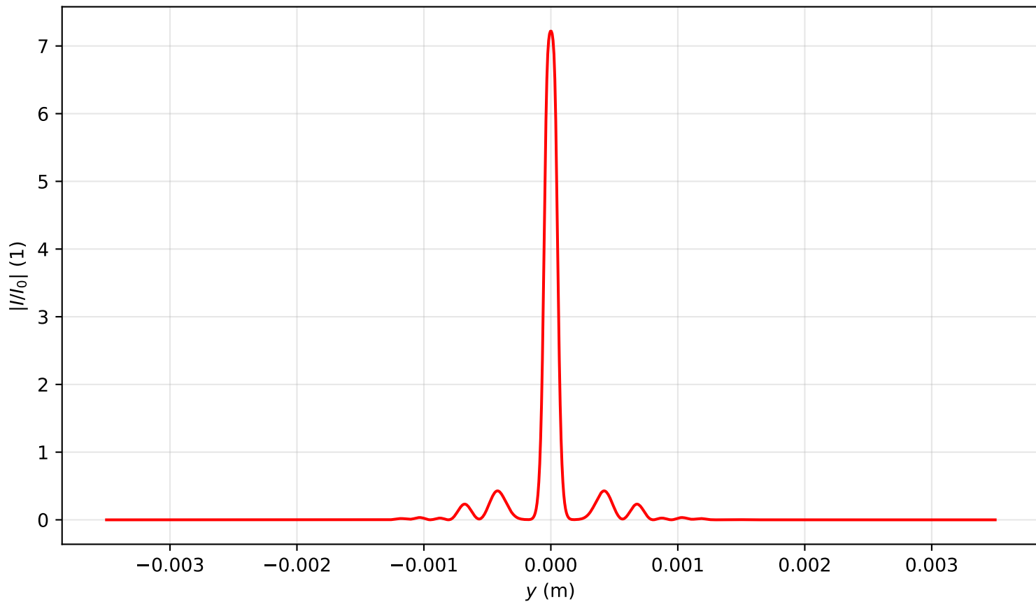
Intensity profile I(x=0, y, z=0.716)/I_0 , P_{in}=15.0P_{cr} , artificial time
