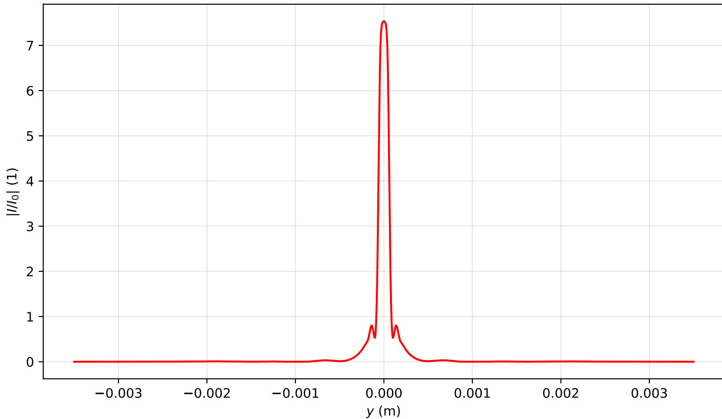
Intensity profile I(x=0, y, z=1.433)/I_0 , P_{in}=15.0P_{cr} , artificial time
