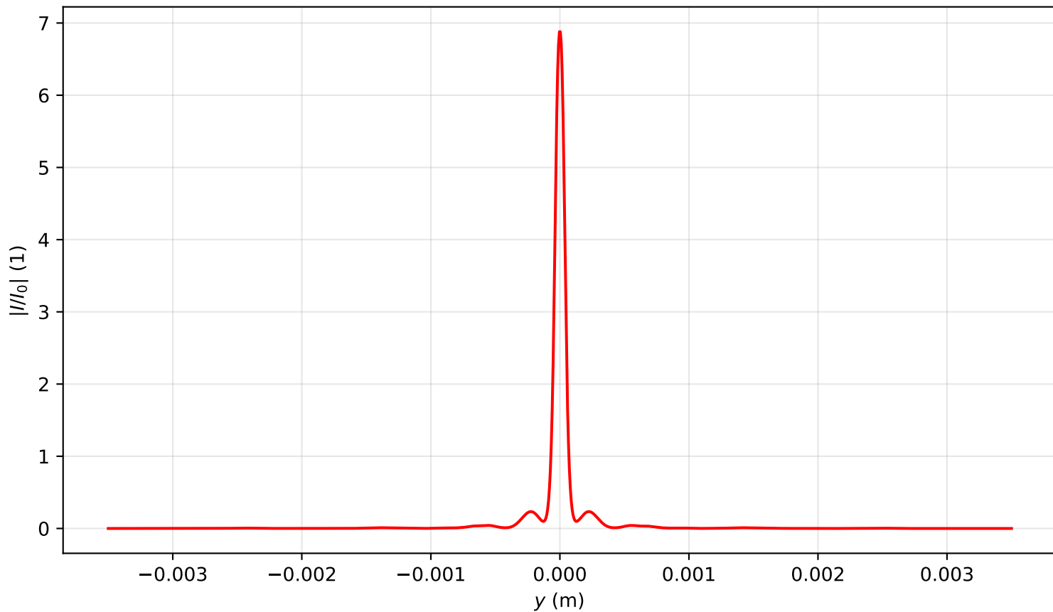
Intensity profile I(x=0, y, z=1.911)/I_0 , P_{in}=15.0P_{cr} , artificial time
