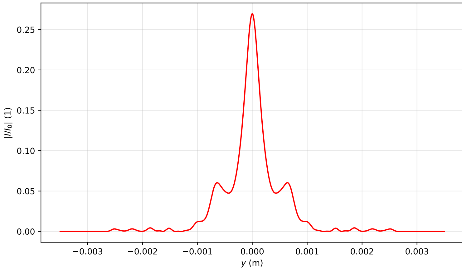
Intensity profile I(x = 0, y, z = 2.388)/I_0 , P_{in}=15.0P_{cr} , artificial time
