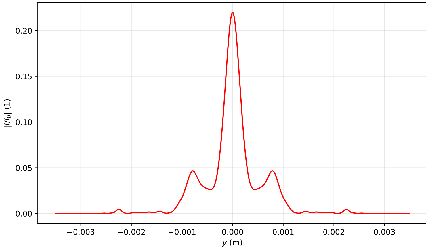
Intensity profile I(x = 0, y, z = 2.627)/I_0 , P_{in}=15.0P_{cr} , artificial time
